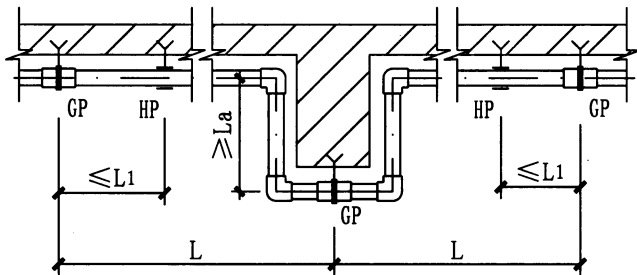
II形补偿
